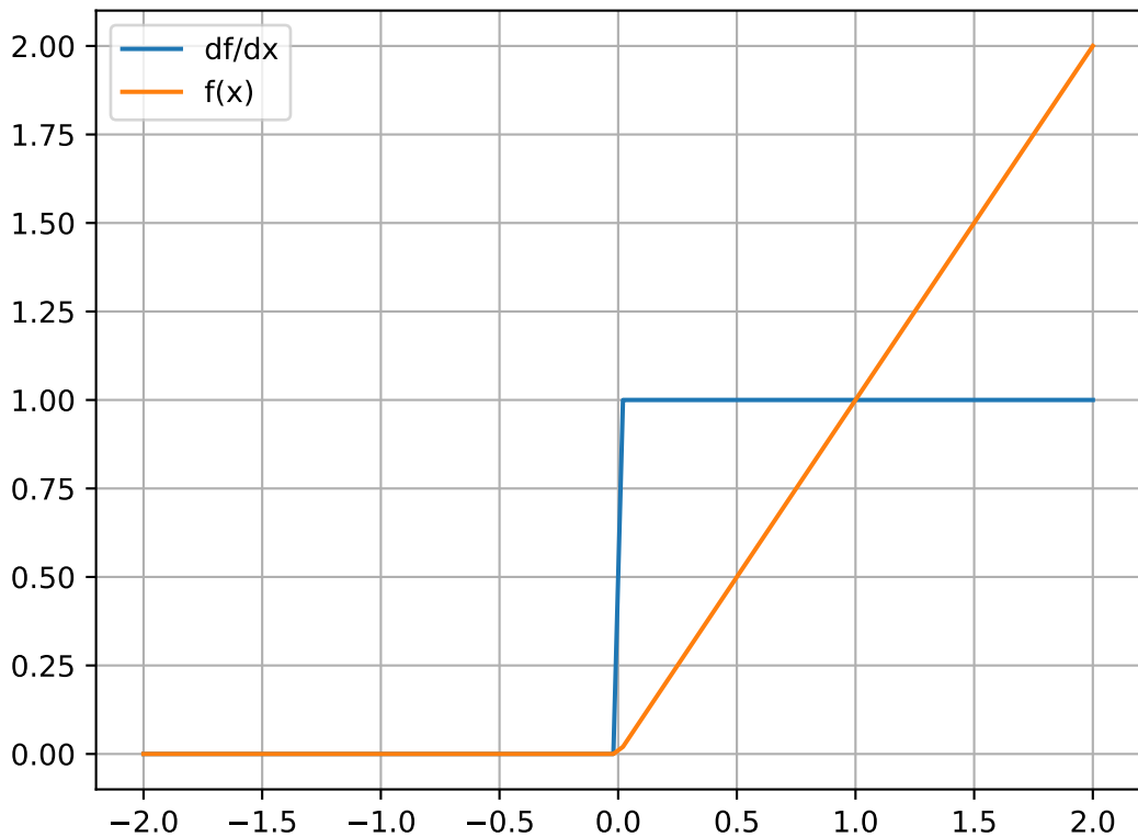
relu(x)
