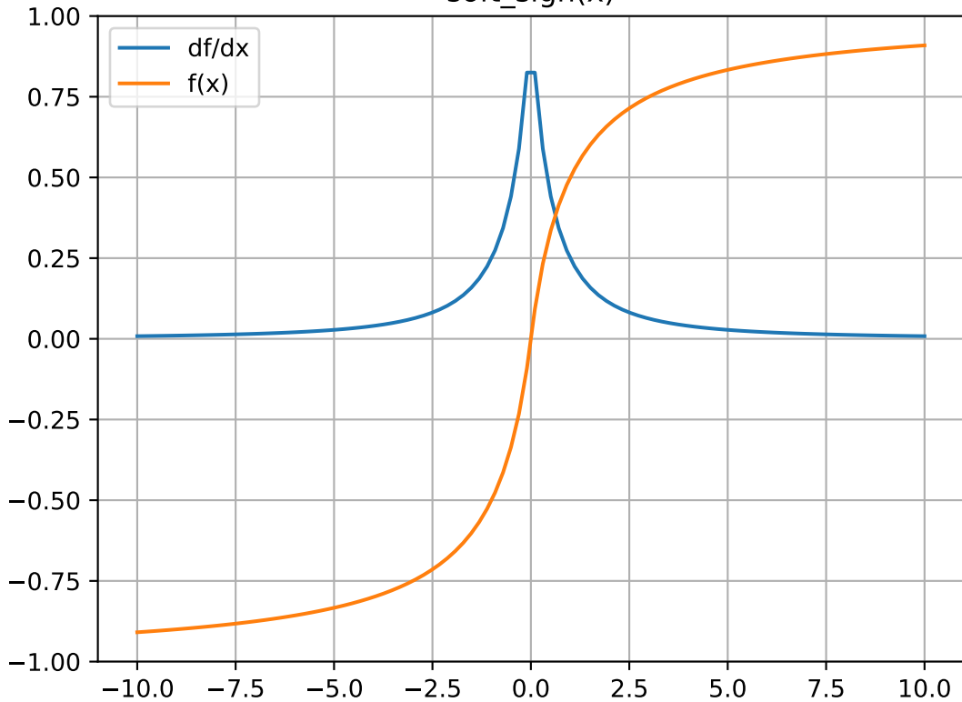
soft_sign(x)
