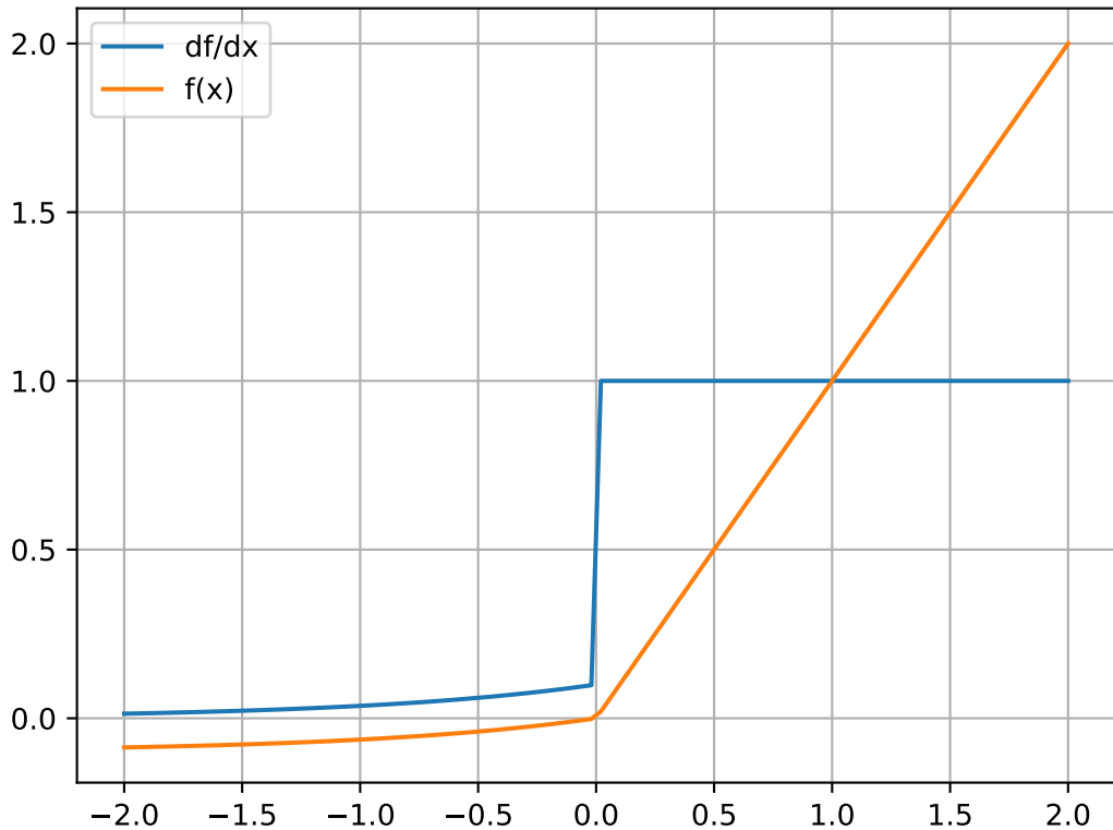
elu(x, alpha=0.1)
